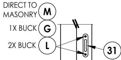
MULTIPOINT TONGUE STRIKE DETAIL
